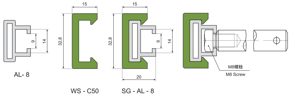
铝轨护栏 SIDE GUIDE WITH ALUMINUM PROFILE
