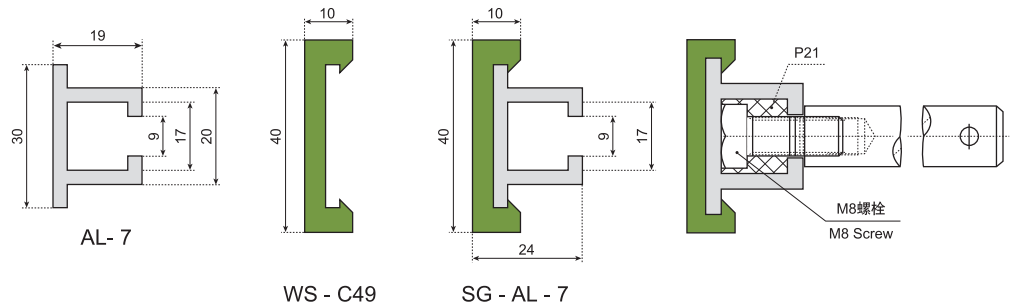
铝轨护栏 SIDE GUIDE WITH ALUMINUM PROFILE
