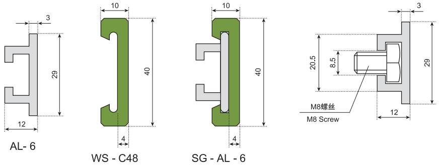
铝轨护栏 SIDE GUIDE WITH ALUMINUM PROFILE
